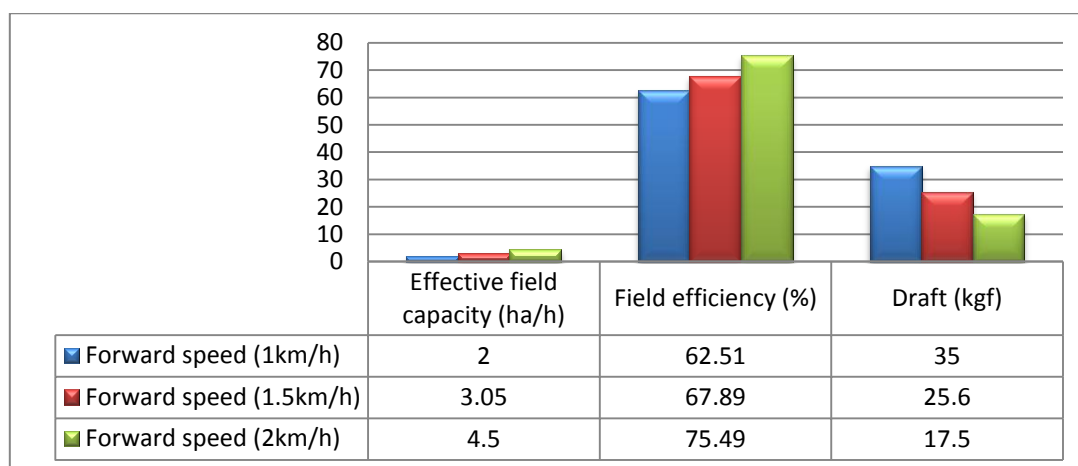
Fig: 4 Effect of Forward speed on Effective field capacity, Field efficiency and Draft load
